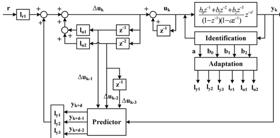
Fig. 6. The simplified GPC control scheme for the 2 nd -order integrating process: Case II.
